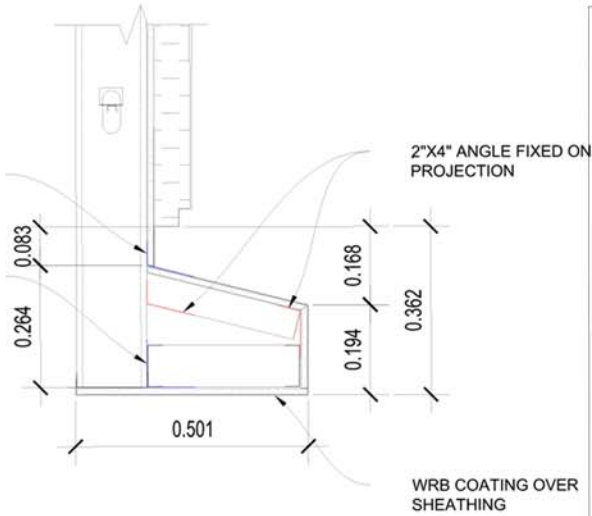
PROJECTION DETAIL @ BOTTOM OF PANEL
