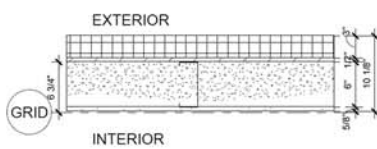
WT3 (EXTERIOR WALL)
